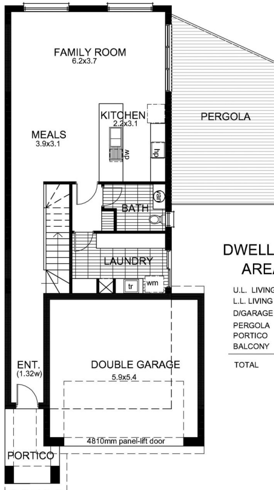
LOWER FLOOR PLAN SCALE 1:100
